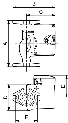
UPS 26-99BFC
